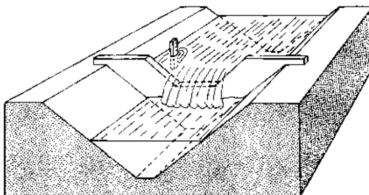
Fig.3.1c (A TRAPEZOIDAL WEIR)
