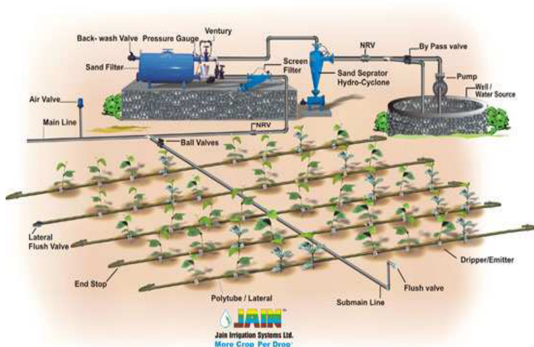
Fig.6.1 (Drip Irrigation Component)
