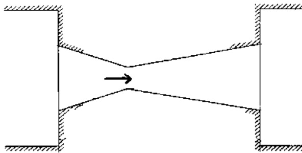
Fig. 3.3 (A cut-throat flume)
