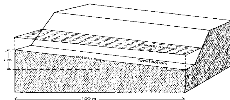
Fig.2.8 (bottom slope of the canal)
