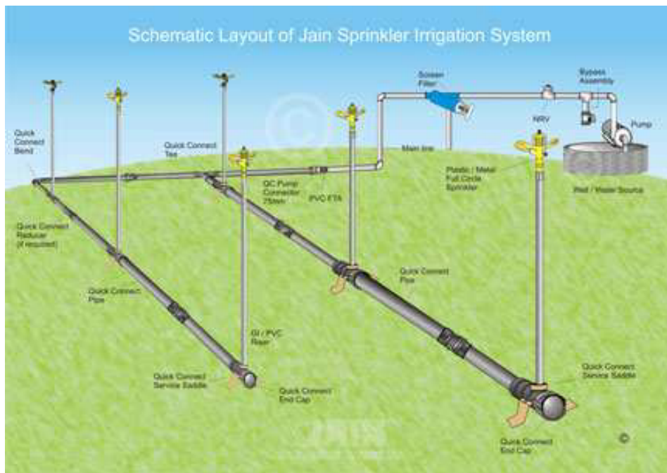
sprinkler irrigation system
