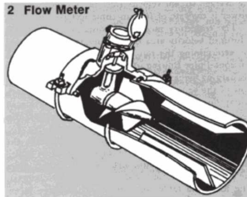
Fig. 3.5 (Flow meter)
