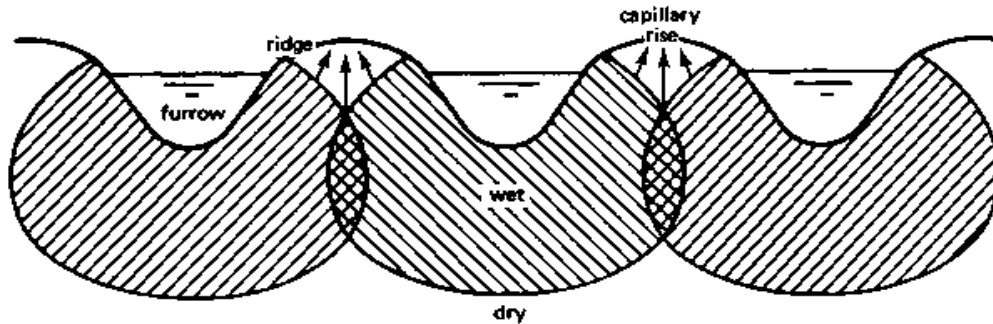
Fig.4.4 (Ideal wetting patterns)
