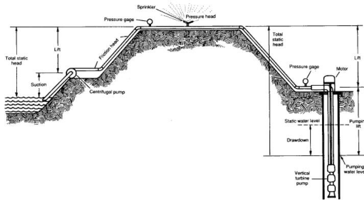
Fig.2.4 (Pumping Lifts)
