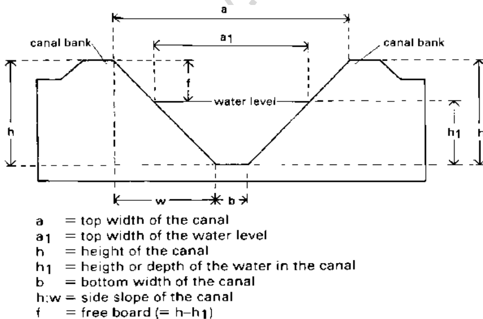
Fig.2.6 (typical cross-section of a trapezoidal canal)
