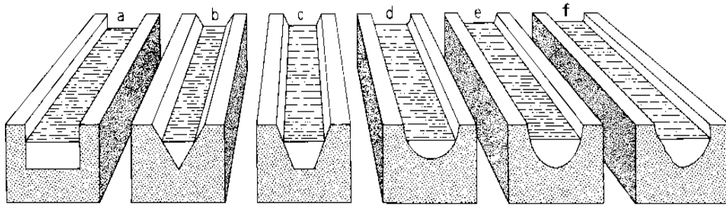
Fig.2.5 (Type of cross-sectional for open canal)
