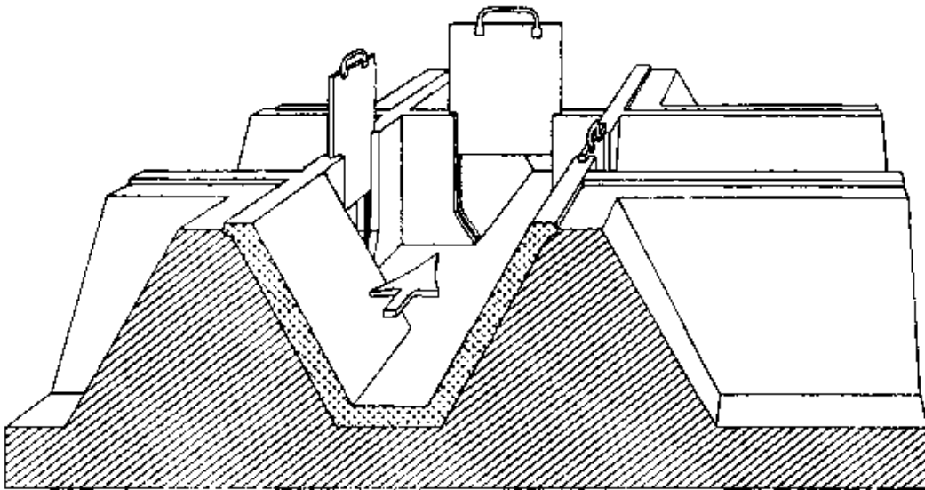
Fig2.12 (A division box with three gates)
