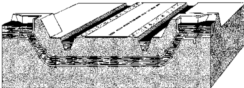
Fig.2.15c (An inverted siphon)
